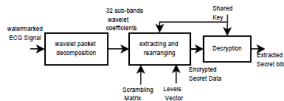
Fig.5. Block diagram of the receiver steganography which includes wavelet decomposition, extraction and decryption
