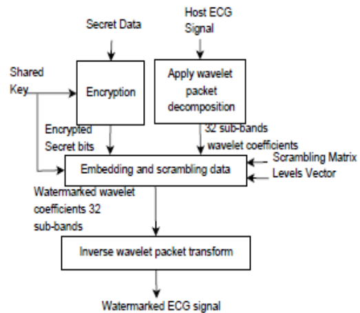
Fig.4. Block diagram of the sender steganography which includes encryption, wavelet decomposition and secret data embedding
