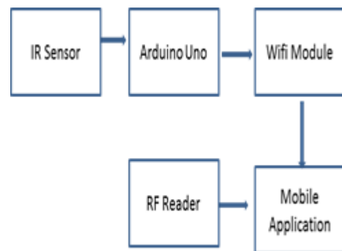
Fig 5.1.Block Diagram of the Proposed System
