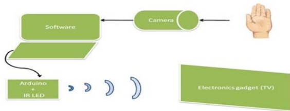
Figure 6 Processing flow
