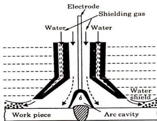
Fig: Underwater Welding Operation
